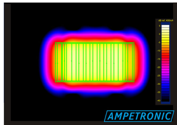
Low Spill Phased Array
