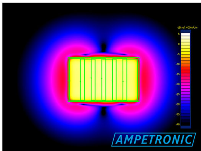
Low Loss Phased Array
